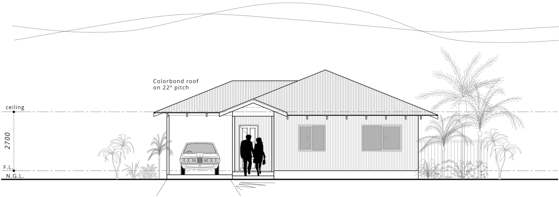
Front Elevation
